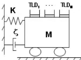
Fig. 2 MTLT
