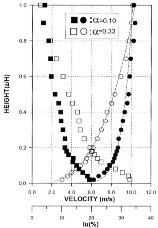
Fig. 7 Vertical distributions of the mean wind speed and turbulence intensities
